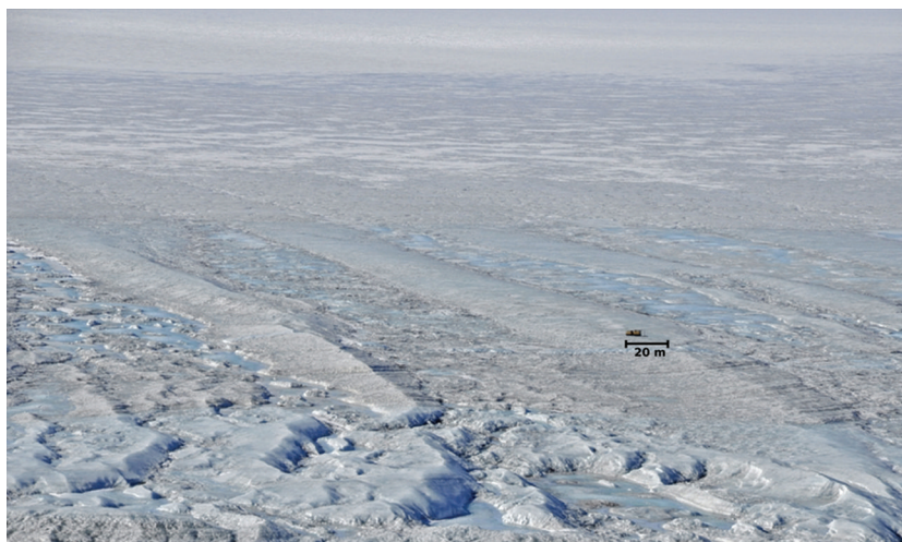
Fig. 2. Marine ice exposed at the ice-shelf surface of SMIS. Photograph was taken in November from Minna Bluff, looking northeast. The Haggglunds vehicle is 7 m long and parked on an ice ridge ~6 m high. Meltwater was observed to pool in elongated ponds between the ridges in December 2010. (Photo: Michael Hambrey.)
